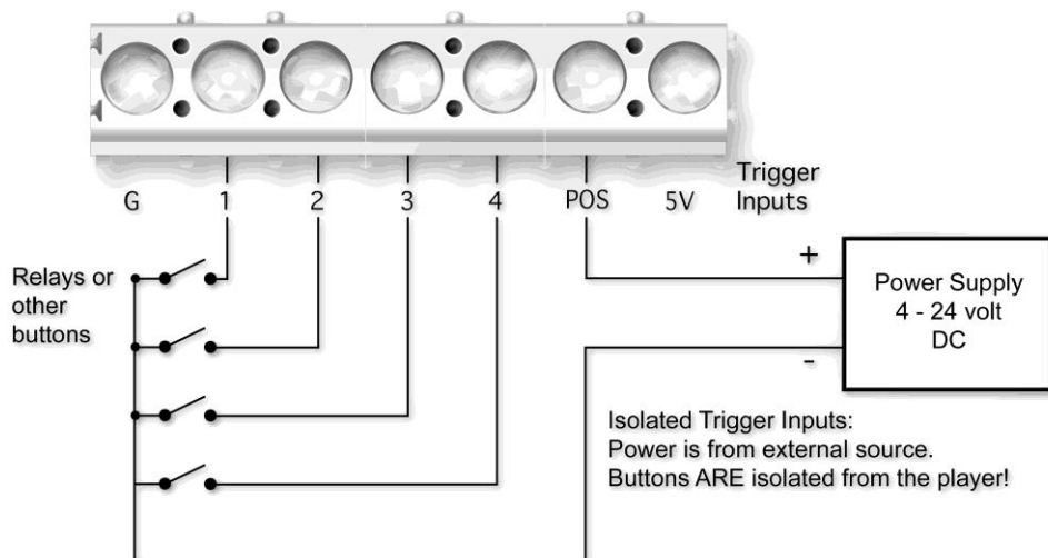
Figure 3 - Isolated Trigger Input Button Connections
