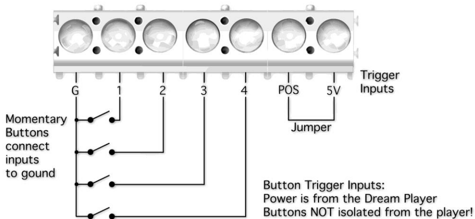
Figure 2 - Simple Trigger Input Button Connections
