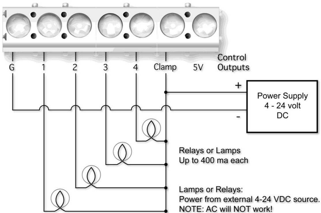
Figure 7 - Lamp/Relay Control Output Connections
