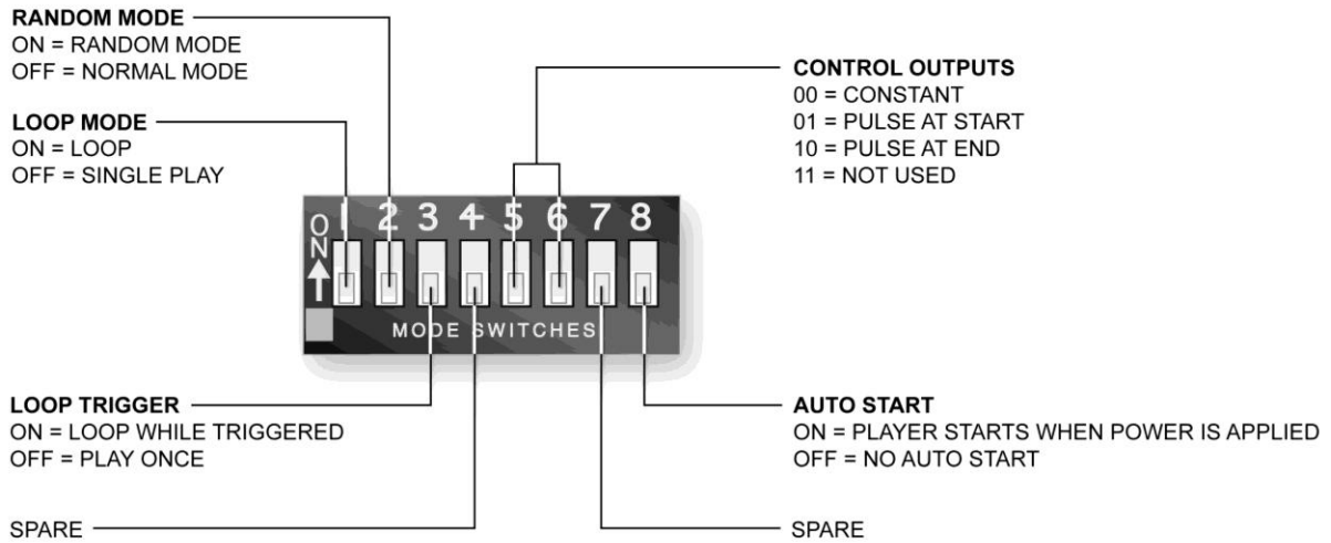
Figure 8 - Mode Switch Settings
