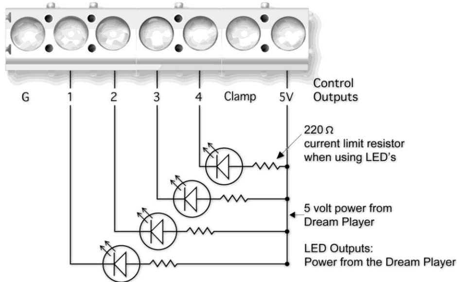
Figure 6 - Simple Control Output LED Connections
